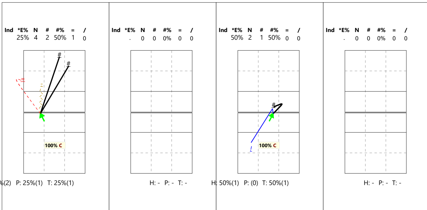
Attack 4 (X7)
